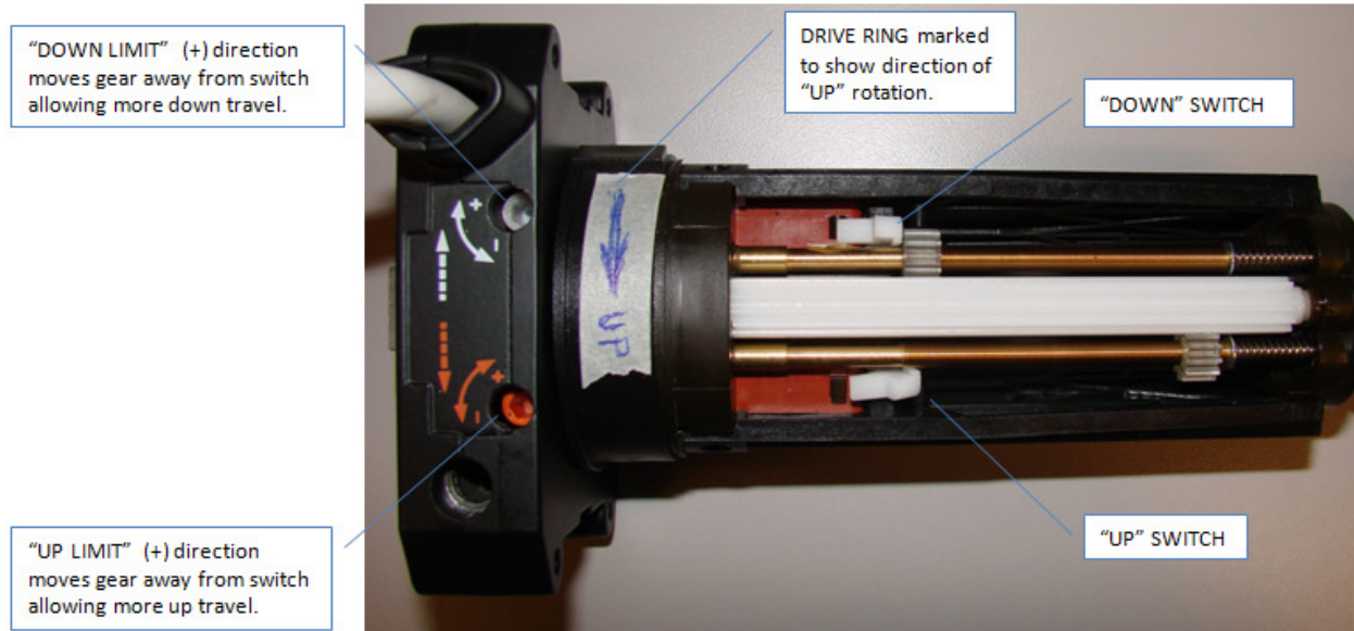
Cutaway view showing micro switches.
