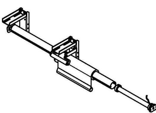
Direct Attach
