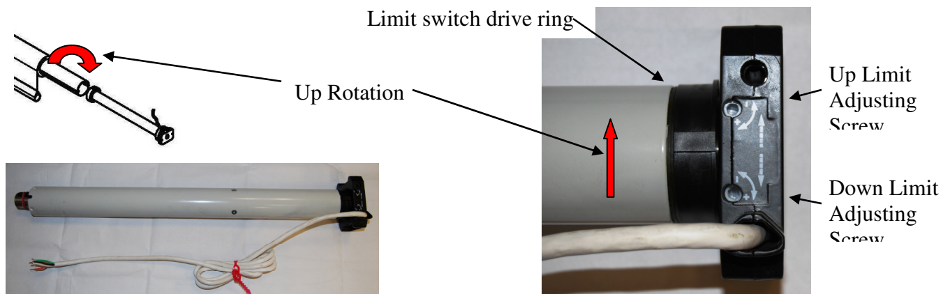
Motor Illustration
