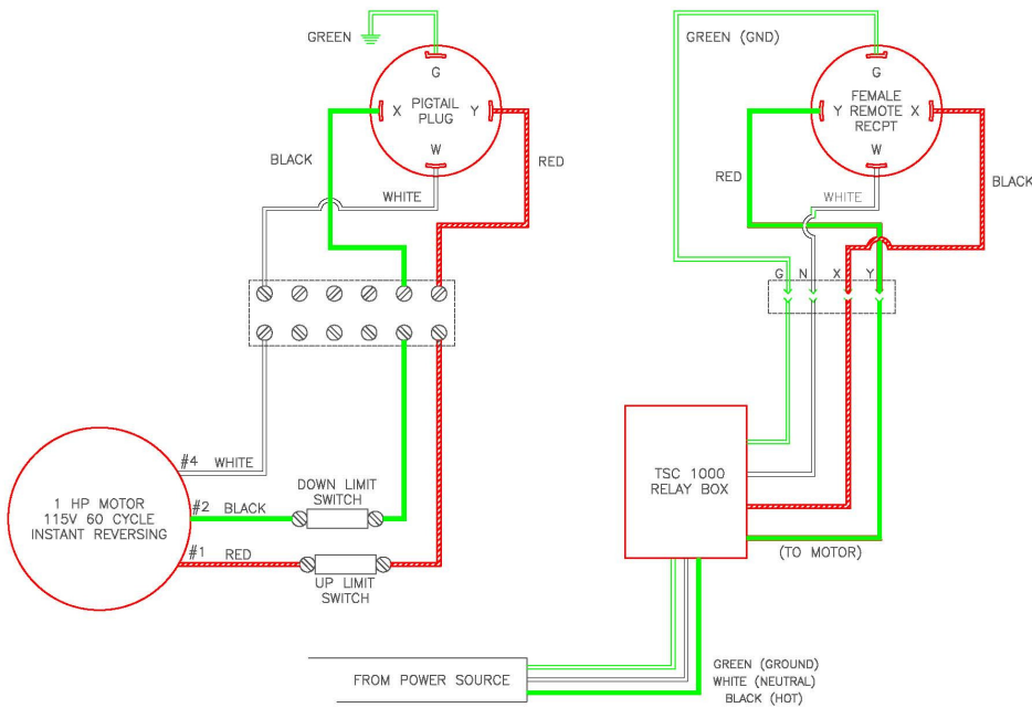
Figure 2. TSC 100 wiring diagram.
