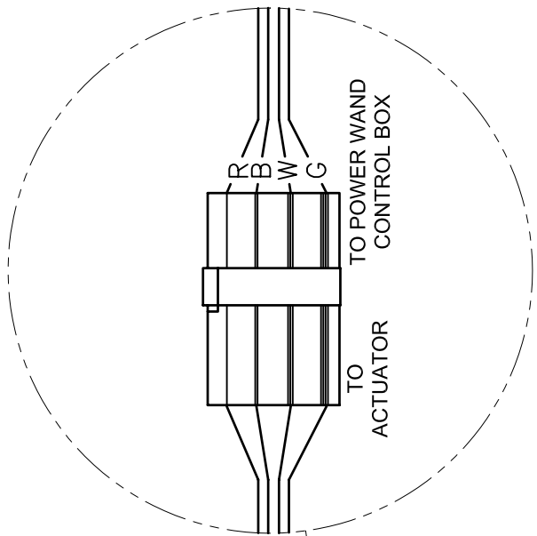
SNAPLOCK PLUG DETAIL
